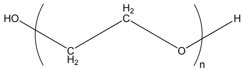
poly(ethylene glycol)
